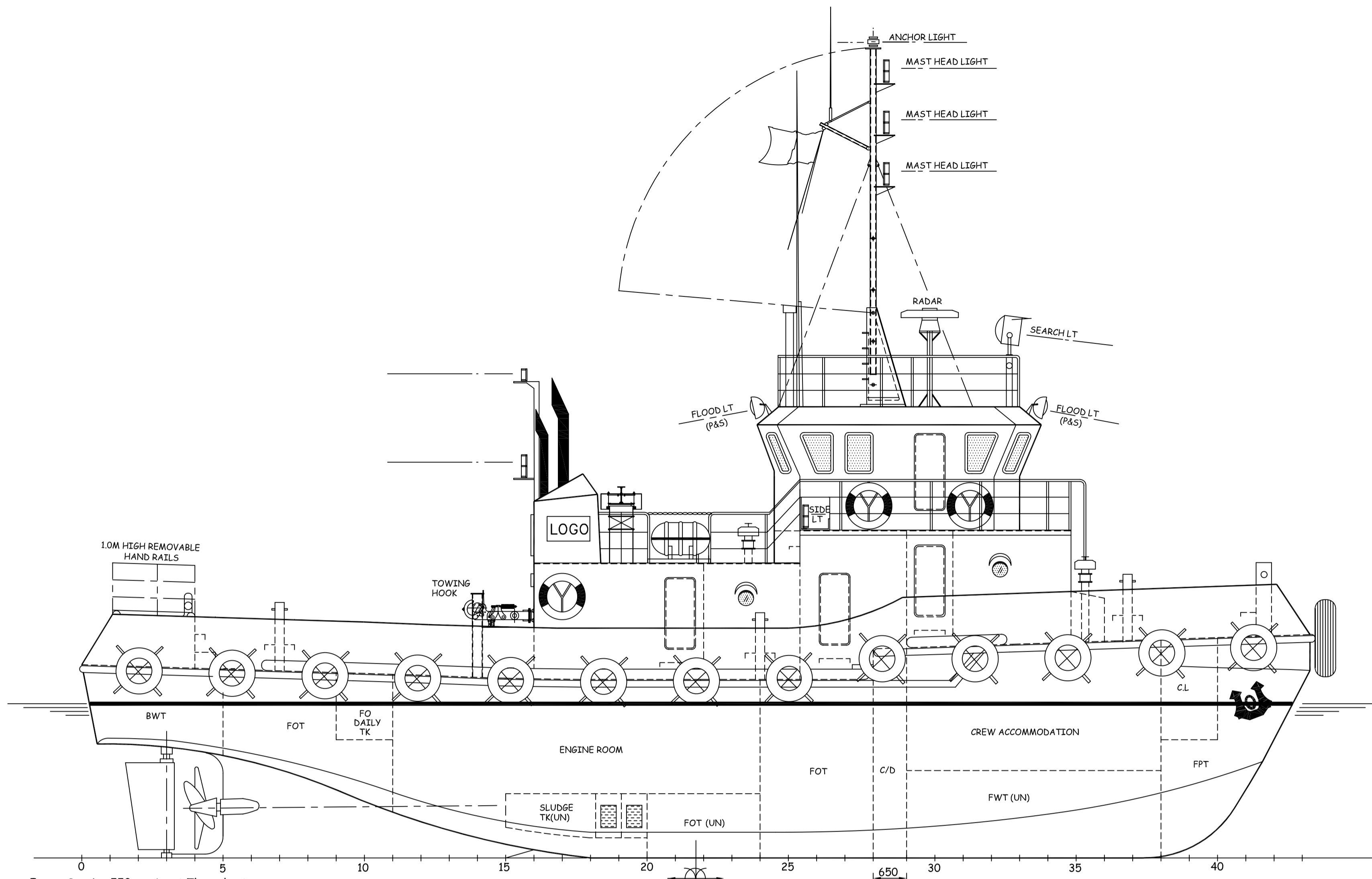
OUTBOARD PROFILE
