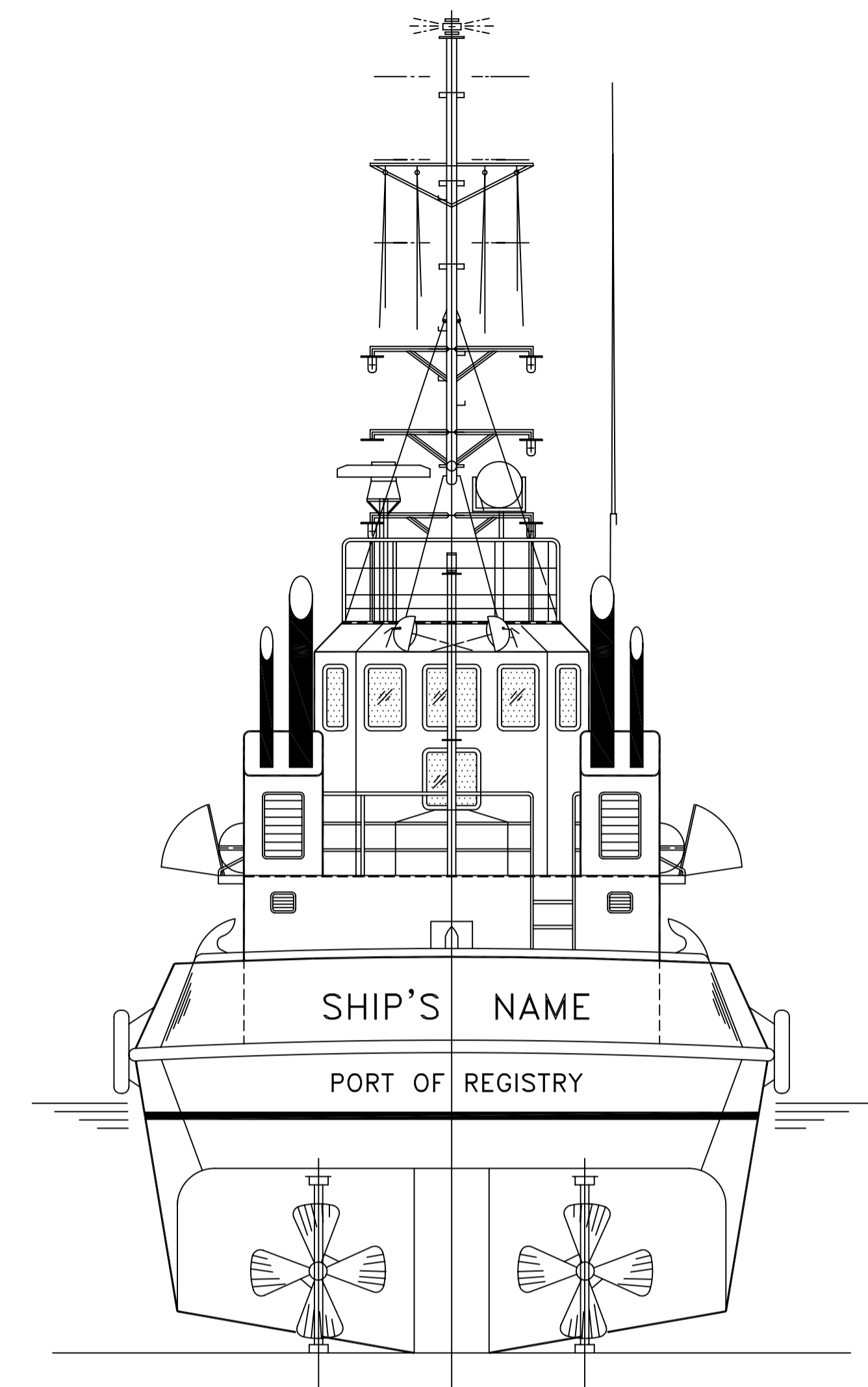
REAR VIEW
